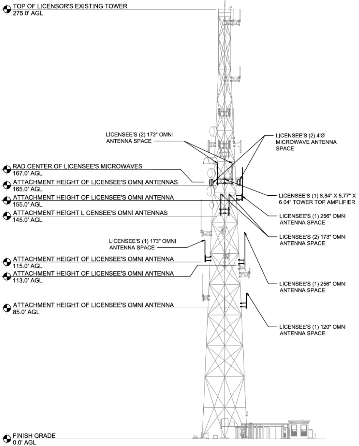
SOUTH ELEVATION
